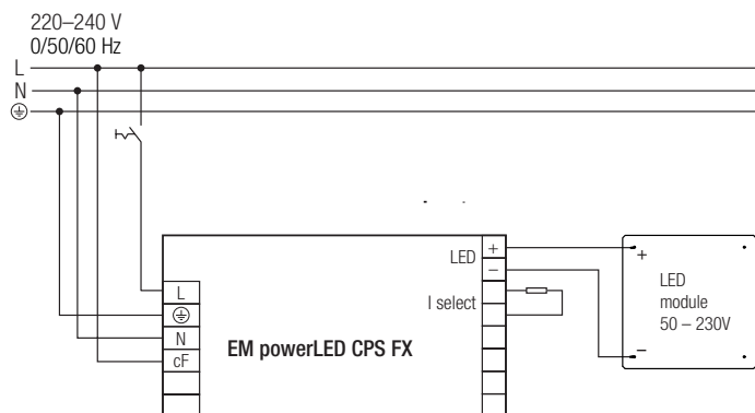
Wiring diagram EM powerLED CPS FX without sensor
