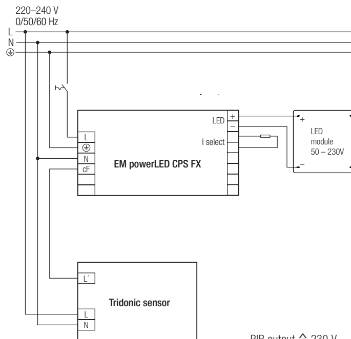
Wiring diagram EM powerLED CPS FX with sensor
