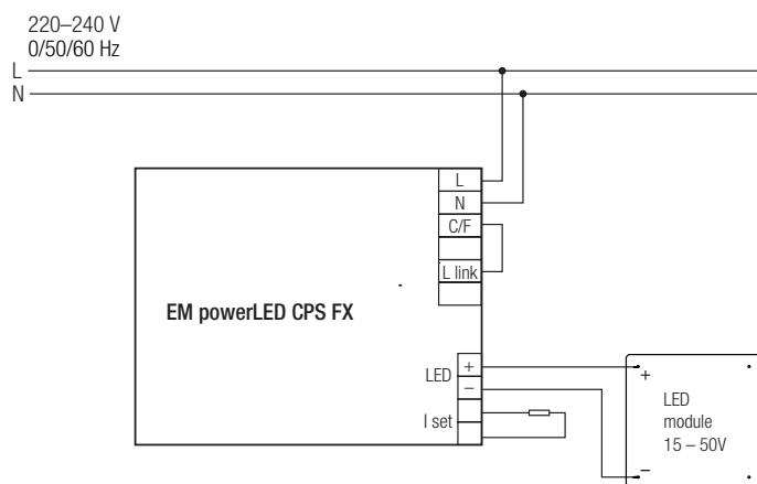
Wiring diagram EM powerLED CPS FX without sensor
