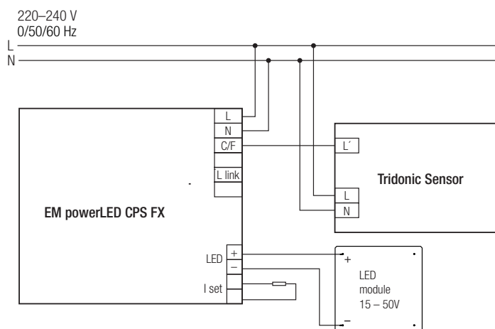
Wiring diagram EM powerLED CPS FX with sensor
