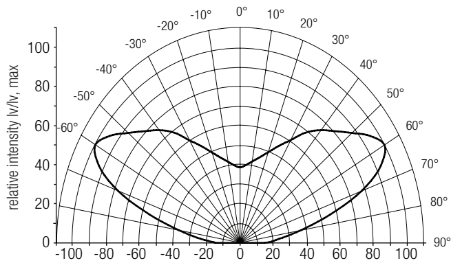
Light distribution I_v/I_{v,max} .
