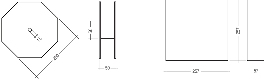
Dimensions roll packaging (packing code 2)
