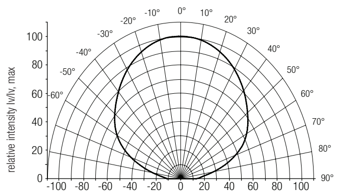
Light distribution I_v/I_{v,max} .
