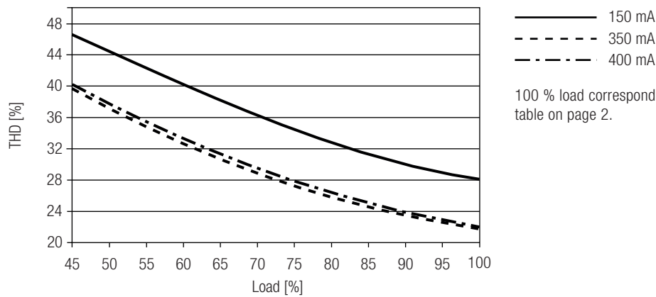
5.3 THD vs load
