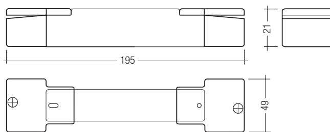
LMAI with strain relief set
