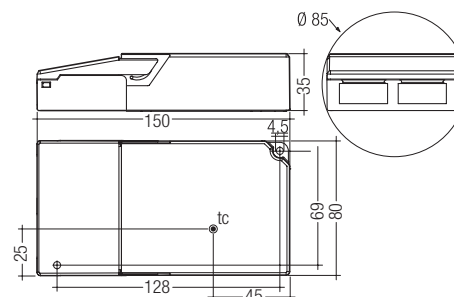
Remote LED Driver
