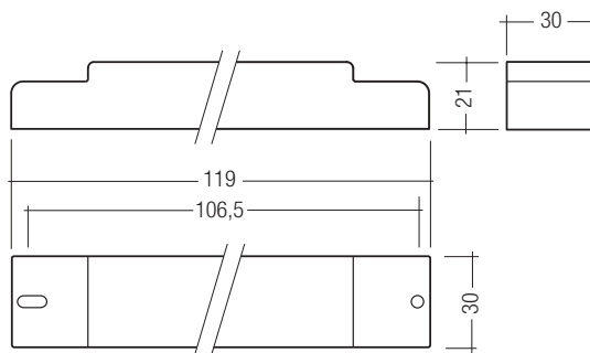
LMAI without strain relief set
