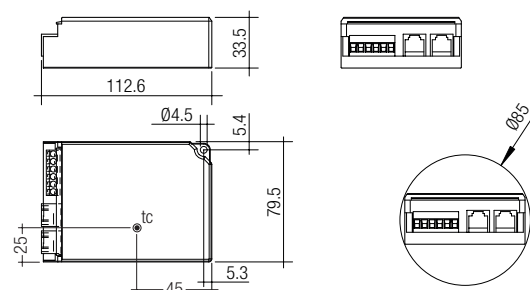
In-built LED Driver
