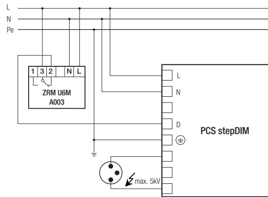
Circuit diagram ZRM U6M A003:
