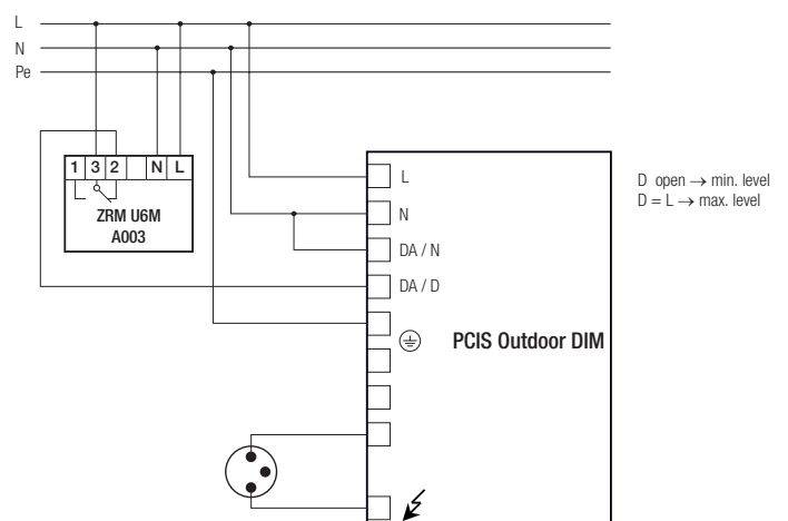
Circuit diagrams for power reduction in HID ECGs
